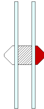
Plant-on Astragal Bars: Outside of the panes
